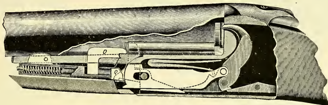
Baker's Ejecting Mechanism.
